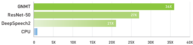
Comparisons made of one NVIDIA Tesla T4 GPU and servers with a dual-socket Xeon Gold 6140 CPU.
